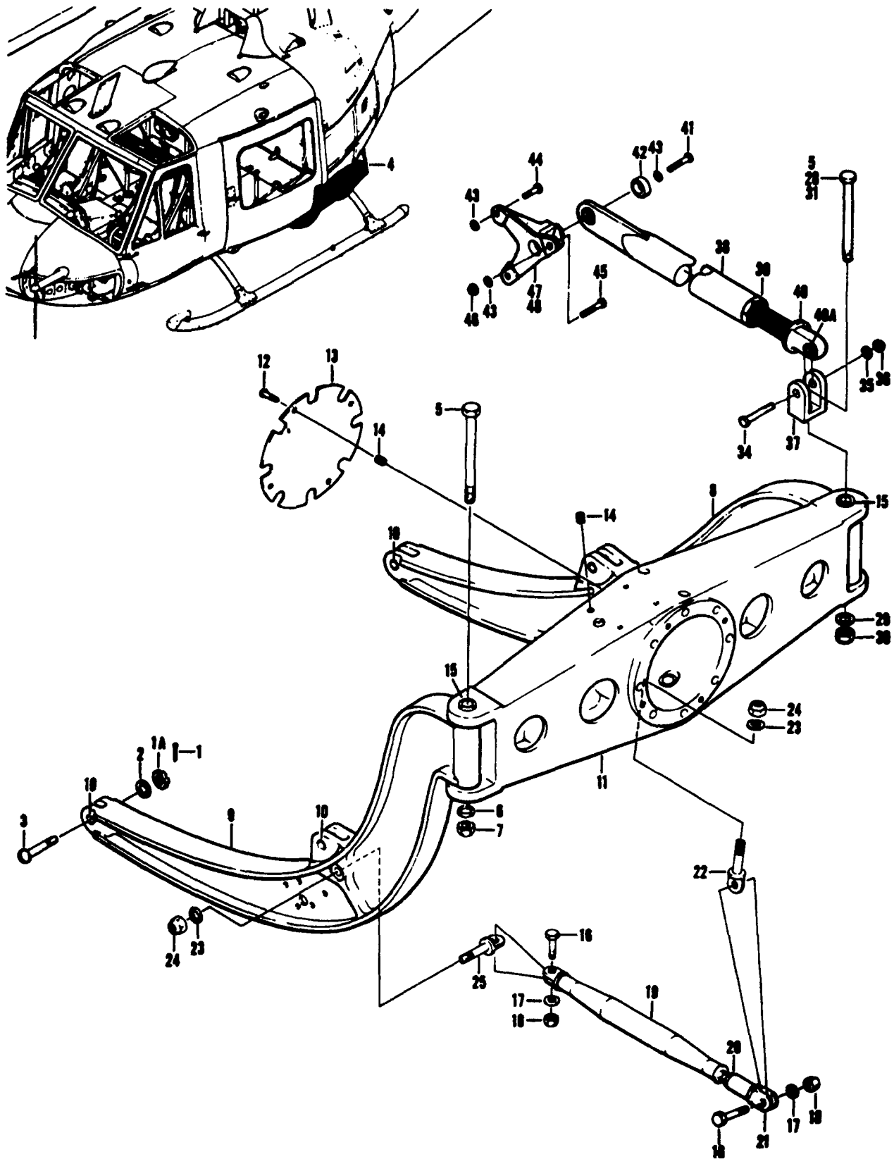
Figure 428. Support Assembly, External Stores
